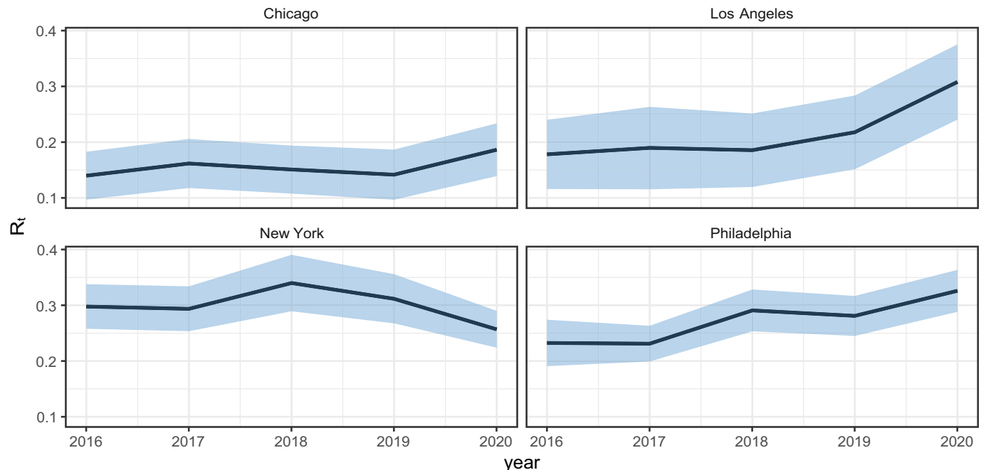
Fig. 4. Estimated dynamic reproduction number, R_t , of shootings for each year along with 95% confidence interval.
