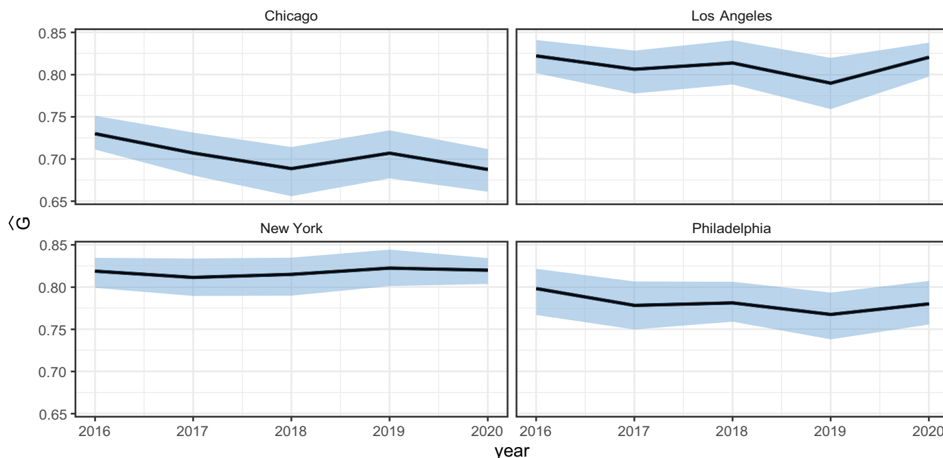
Fig. 5. Estimated yearly Gini index, G , of shootings using a grid of 500 m \times 500 m cells. 95% confidence interval shown in blue. (For interpretation of the references to colour in this figure legend, the reader is referred to the web version of this article.)
