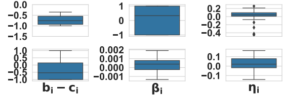
Figure 5: The estimates of b_i - c_i , \beta_i and \eta_i . Top : the homicides data aggregated with T = 60 . Bottom : the bilateral trading data.
